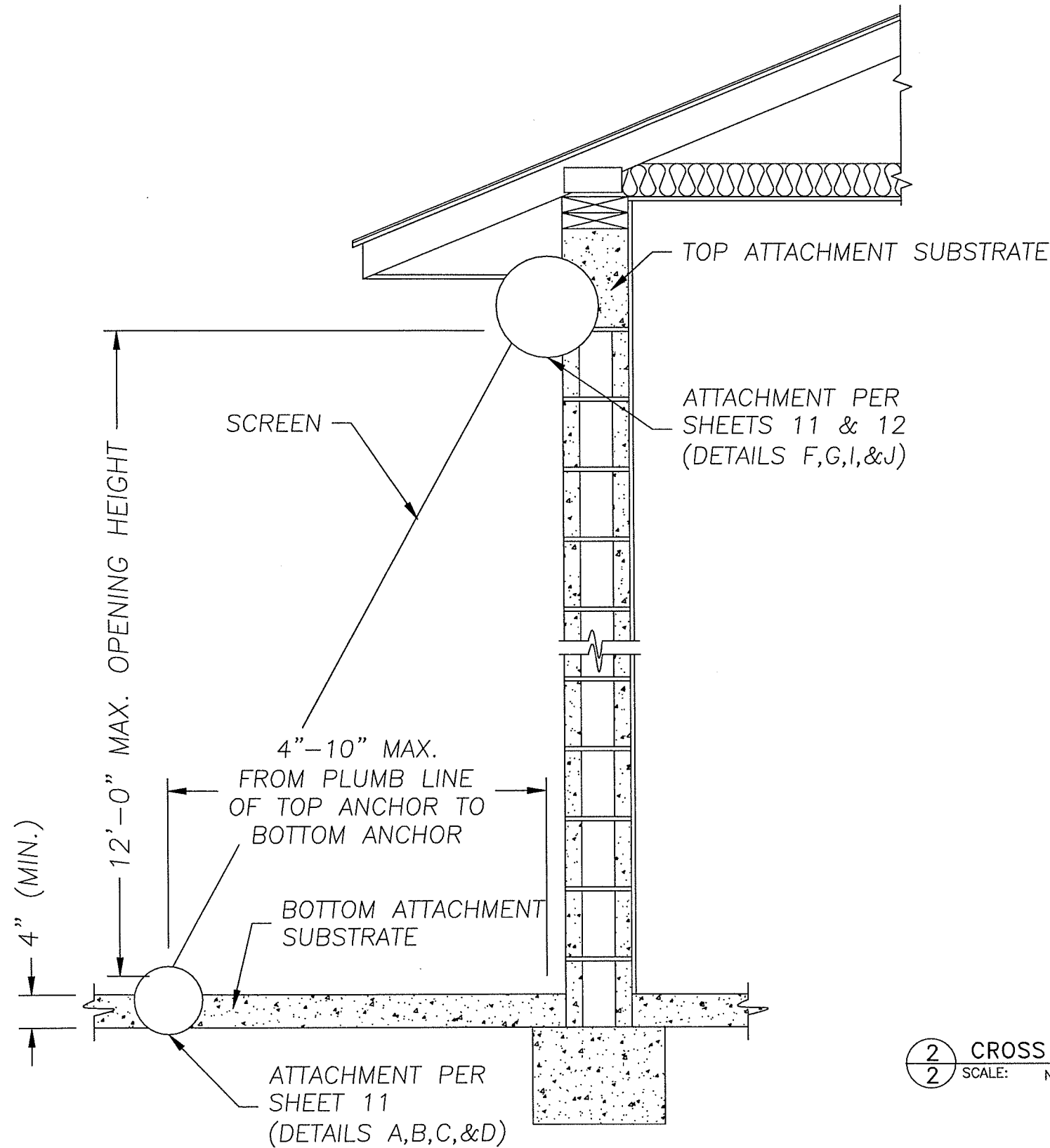
1 SECTION VIEW OF ANGLE MOUNTED SCREEN 2 SCALE: NTS = 1'-0"
