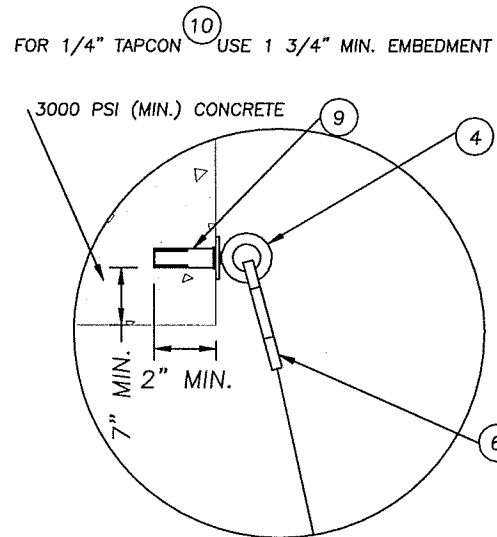
DETAIL "E" SCREEN TO CONCRETE @ TOP DROP-IN FASTENER IS INSTALLED HORIZONTALLY ON INSIDE OF OPENING (USE MIN. EDGE DISTANCE)
