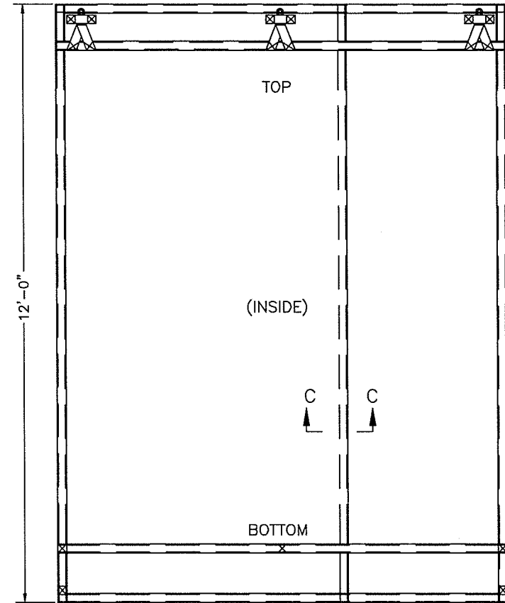
HURRICANE SCREEN ELEVATION (INSIDE STITCHING DETAILS. THE SCREEN IS MANUFACTURED IN (3) STYLES; VERTICAL SEAM, HORIZONTAL SEAM, & NON-SEAMED OVERLAPPED FABRIC PANELS)
