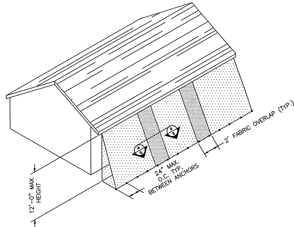
1 ANGLED SCREEN OVERLAP - IN APPLICATION 6 SCALE: NTS=1'-0"
