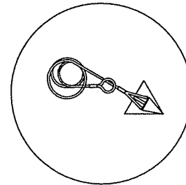
DETAIL "M" 10" MALLEABLE IRON EARTH ANCHOR 3/8" GALVANIZED AIRCRAFT CABLE, 72" LONG. BY AMERICAN EARTH ANCHORS OR EQUAL
