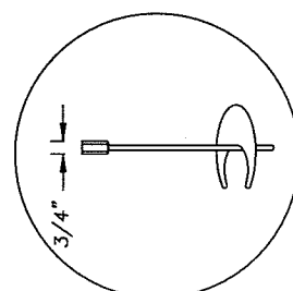
DETAIL "O" 1/2" SCREW-IN EARTH ANCHOR WITH 4" HELIX, 30" LONG. (NUT ATTACHMENT) BY MINUTE MAN PRODUCTS OR EQUAL
