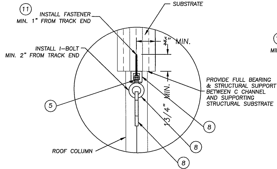
DETAIL "A" SCREEN TO TRACK @ TOP FASTENER IS INSTALLED HORIZONTALLY (USE MIN. EDGE DISTANCE)
