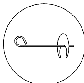
DETAIL "N" 1/2" SCREW-IN EARTH ANCHOR WITH 4" HELIX, 30" LONG. BY MINUTE MAN PRODUCTS OR EQUAL
