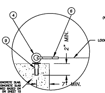
DETAIL "H" SCREEN TO CONCRETE TOP [LOOP END] DROP-IN FASTENER IS INSTALLED HORIZONTALLY ON INSIDE OF OPENING (USE MIN. EDGE DISTANCE)
