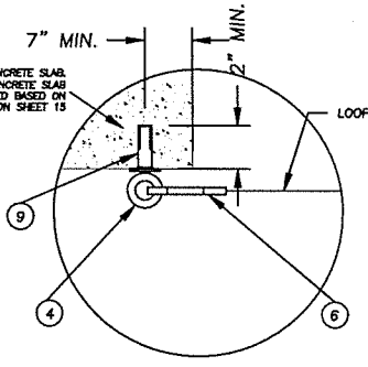
DETAIL "I" SCREEN TO CONCRETE TOP [LOOP END] DROP-IN FASTENER IS INSTALLED HORIZONTALLY ON OUTSIDE OF OPENING (USE 2" MIN. EDGE DISTANCE)
