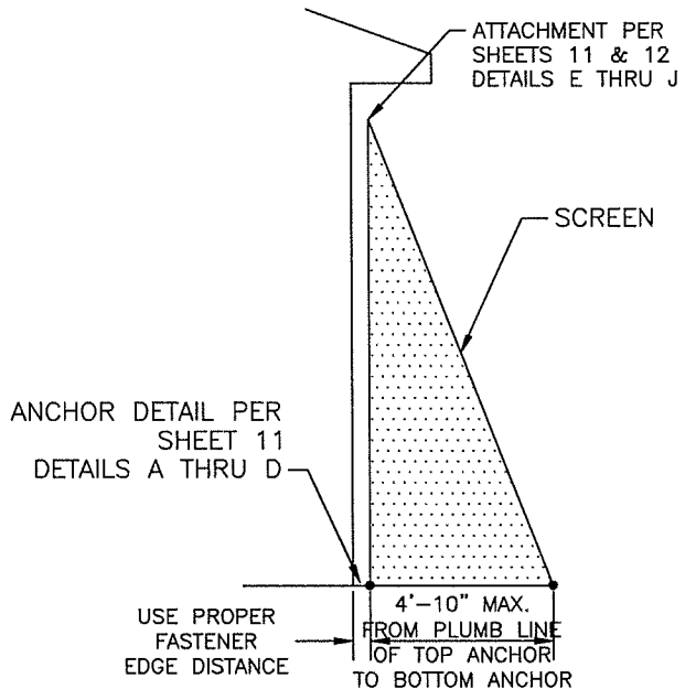
3 3 SIDE CLOSURE SCREEN SCALE: NTS = 1'-0"
