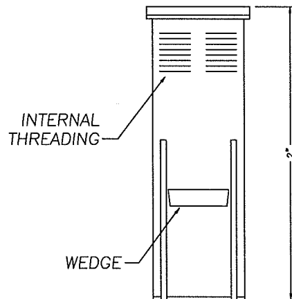
⑨ Ø1/2" DROP-IN ANCHOR STAINLESS STEEL
