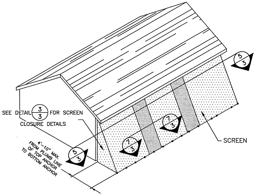
1 3 SCREEN WITH SIDE CLOSURE SCREEN SCALE: NTS = 1'-0"
