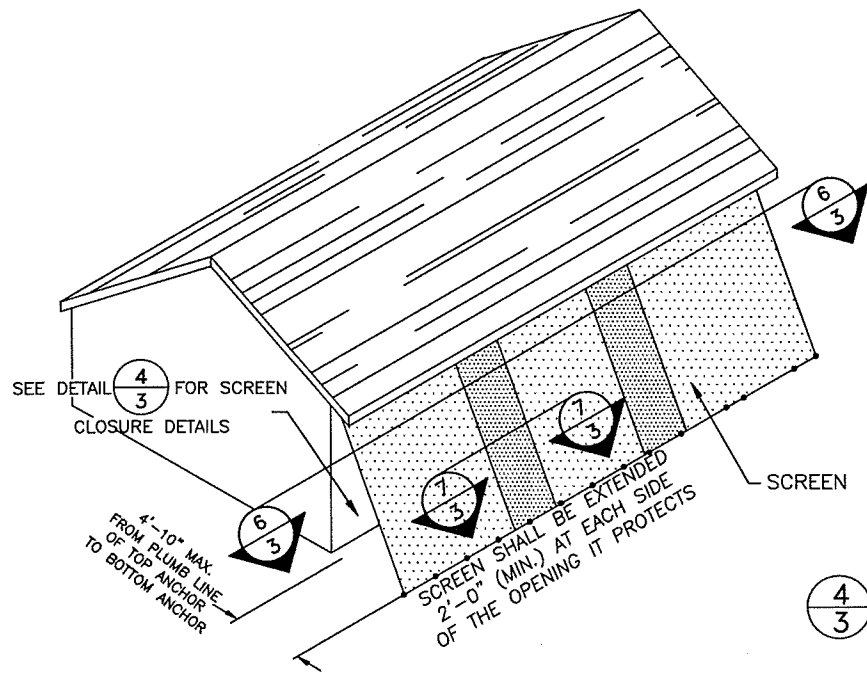
2 3 SCREEN WITHOUT SIDE CLOSURE SCREEN SCALE: NTS = 1'-0"
