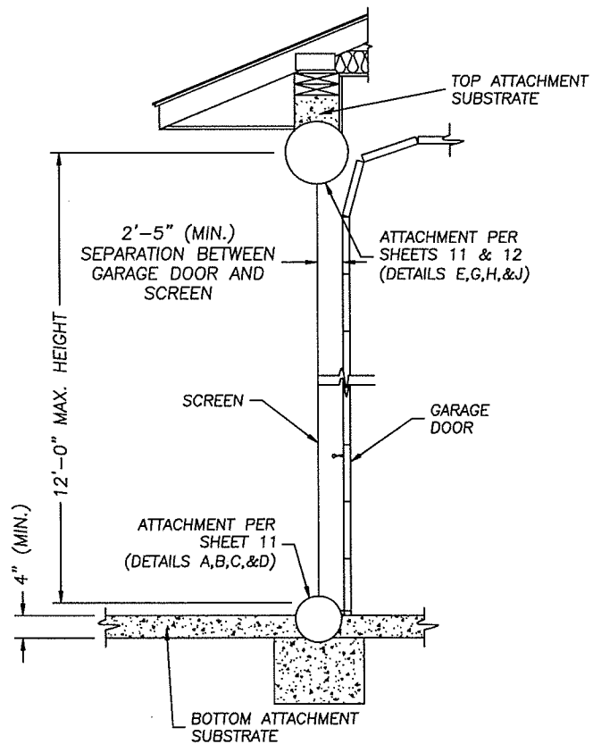
2 CROSS SECTION OF VERT. MOUNTED STRAIGHT DROP SCREEN (SIDE VIEW/GARAGE DOOR) 4 SCALE: NTS = 1'-0"
