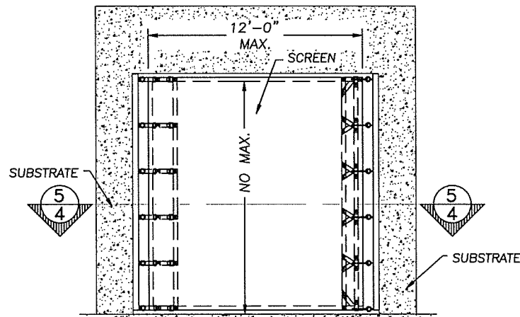
4 HOR. MOUNTED STRAIGHT DROP SCREEN (ELEVATION) 4 SCALE: NTS = 1'-0"
