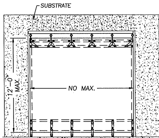
1 CROSS SECTION OF VERT. MOUNTED STRAIGHT DROP SCREEN (SIDE VIEW)/LANAI 4 SCALE: NTS = 1'-0"
