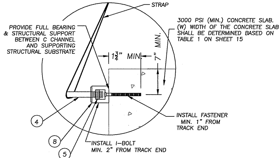
DETAIL "C" SCREEN TO TRACK @ BOTTOM TAPCON FASTENER IS INSTALLED HORIZONTALLY (USE MIN. EDGE DISTANCE)
