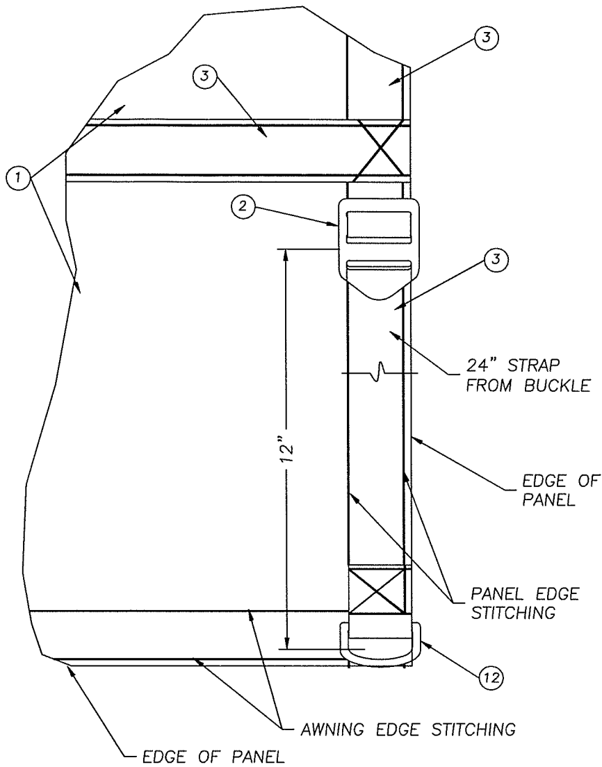
STITCHING DETAIL
