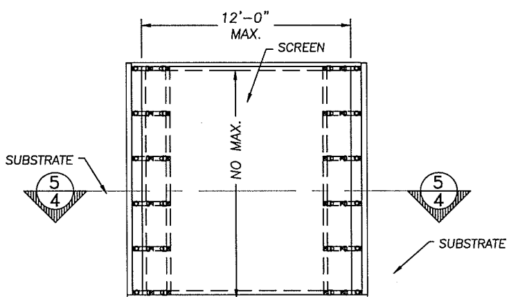
4.1 HOR. MOUNTED STRAP AND BUCKLE (ELEVATION) OPTION 2 4 SCALE: NTS = 1'-0"
