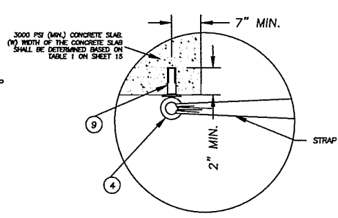
DETAIL "L" SCREEN TO CONCRETE TOP [STRAP END] DROP-IN FASTENER IS INSTALLED HORIZONTALLY ON OUTSIDE OF OPENING (USE 2" MIN. EDGE DISTANCE)
