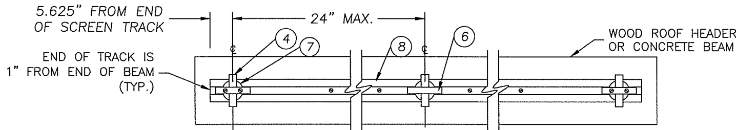
3 7 PLAN VIEW (LOOKING UP) TOP VERTICAL MOUNTING IN WOOD OR CONCRETE SCALE: NTS = 1'-0"
