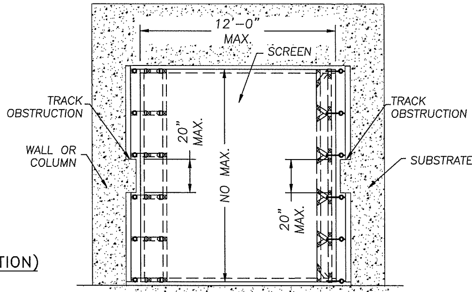
2 7 HOR. MOUNTED SCREEN W/ TRACK OBSTRUCTION (ELEVATION) SCALE: NTS = 1'-0"
