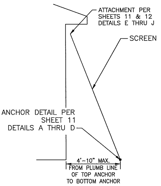
4 3 SIDE CLOSURE SCREEN - NO RETURN SCALE: NTS = 1'-0"
