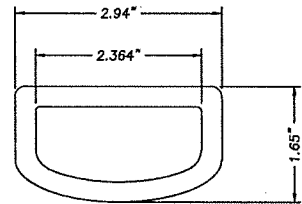
⑫ LADDERLOC LOOP .161" THK. ACETAL HOSTAFORM C
