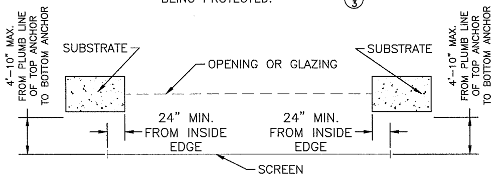
6 3 ANGLED SCREEN CLOSURE - NO RETURN (PLAN VIEW) SCALE: NTS = 1'-0"
