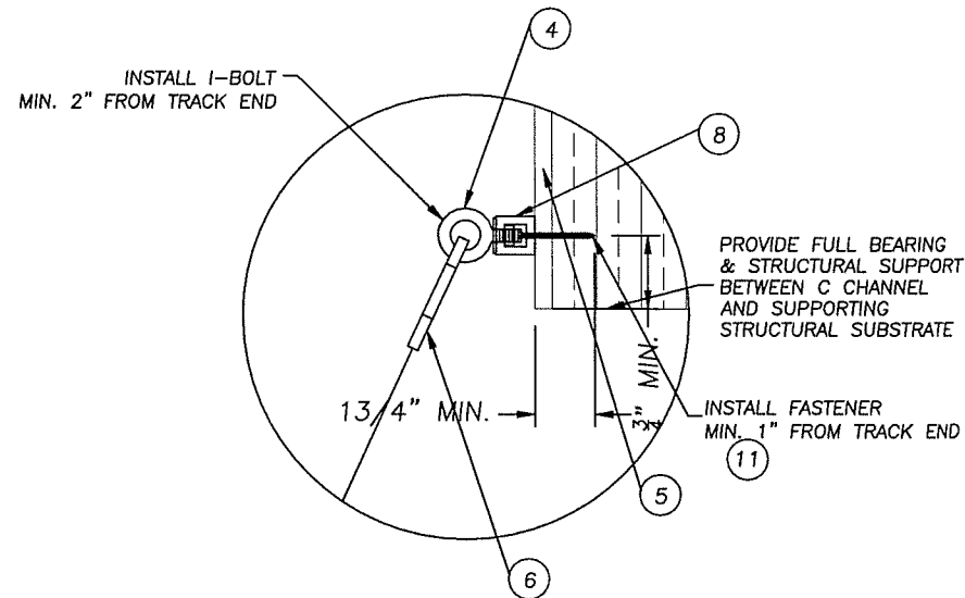
DETAIL "C" SCREEN TO TRACK @ TOP FASTENER IS INSTALLED HORIZONTALLY ON OUTSIDE OF OPENING (USE MIN. EDGE DISTANCE)
