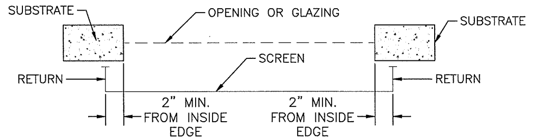
5 3 ANGLED SCREEN CLOSURE WITH RETURN (PLAN VIEW) SCALE: NTS = 1'-0"
